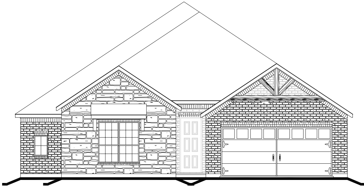
ELEVATION "B"
