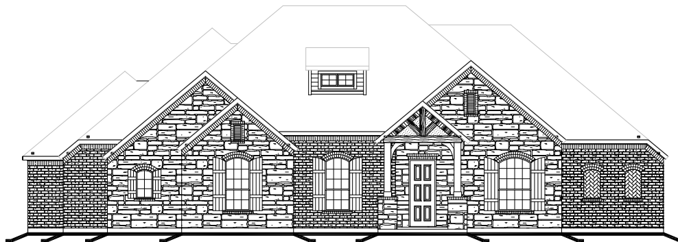
ELEVATION "B"
