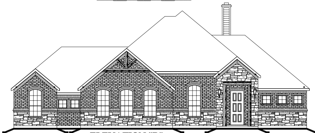
ELEVATION "B"
