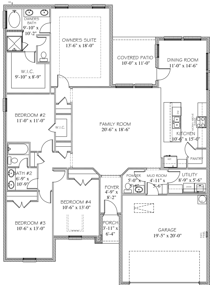
FLOOR PLAN
