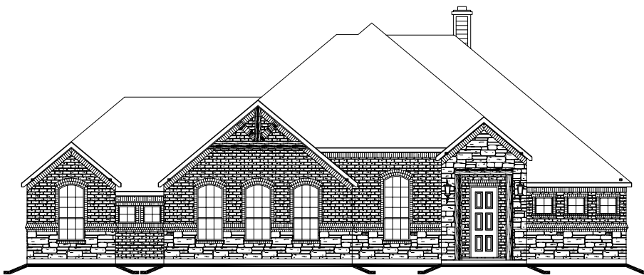
ELEVATION "B"
